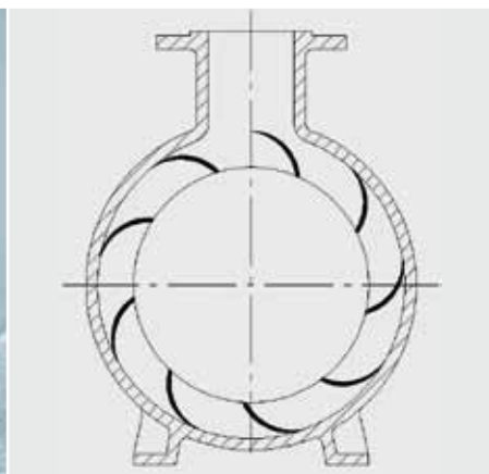
Diffuser Casing
