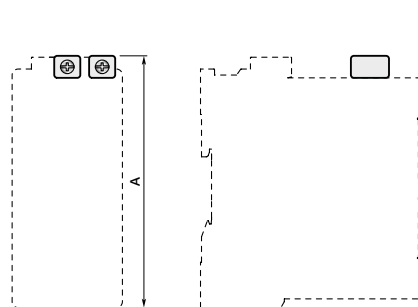
LK96-4F or LK96-4L on AF40 ... AF96
