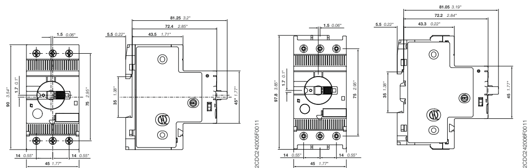
MO132 ≤ 10 A
