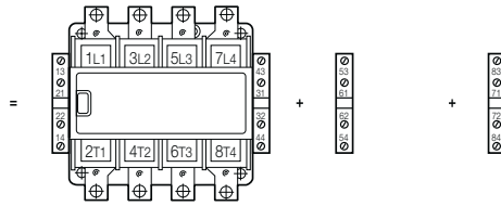
= EK550, EK1000-40-22 + CAL16-11C + CAL16-11D
