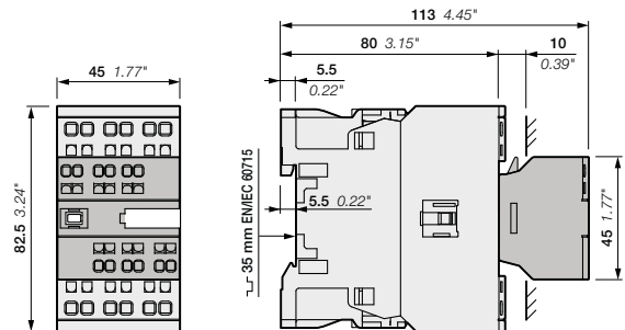
AF26..S + CAT4..S 2-pole auxiliary contact and coil terminal block
