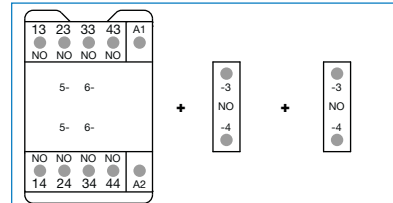
Combination 60E = NS40E + CA3-10 + CA3-10
