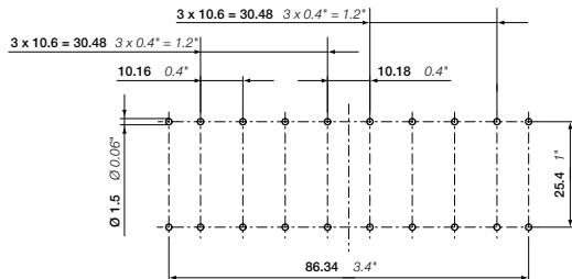
Mini reversing contactors with soldering pins
