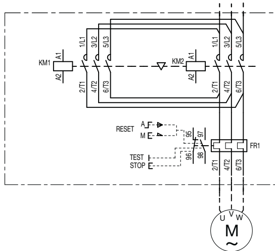
Power circuit
