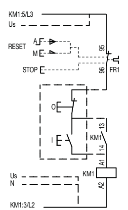
AC or DC remote control
