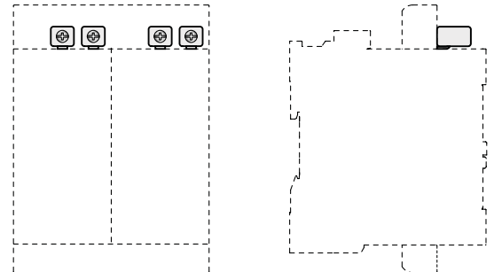
LK96-4B on AF40 ... AF96 using BER or BEY connection sets
