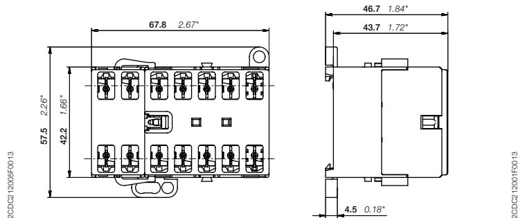
Mini contactors or contactor relays + CA6-11E-F, CA6-11M-F, CA6-11N-F
