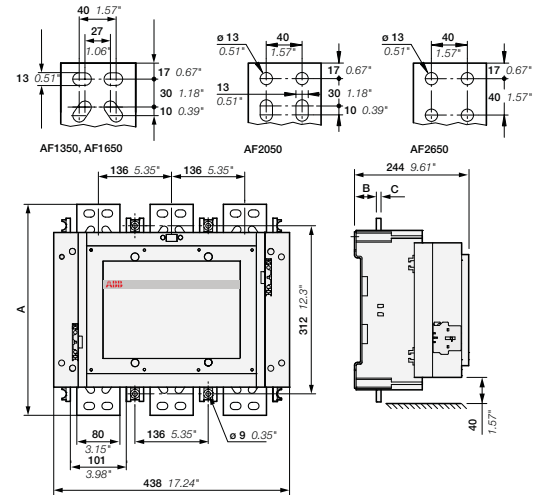
AF1350, AF1650, AF2050, AF2650
