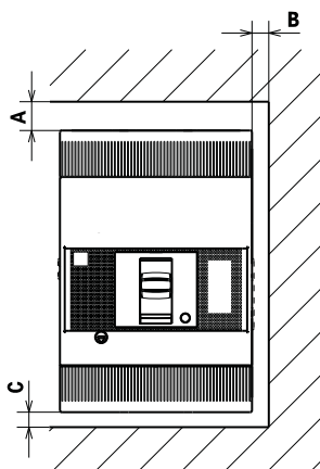
MO5100, insulation distances
