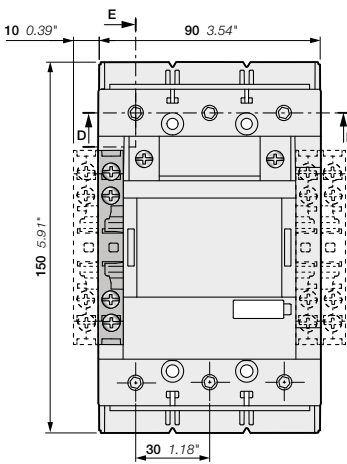
AF116, AF140, AF146-30-00 + CAL19 2-pole auxiliary contact block AF116, AF140, AF146-30-11
