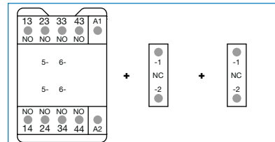
Combination 42E = NS40E + CA3-01 + CA3-01
