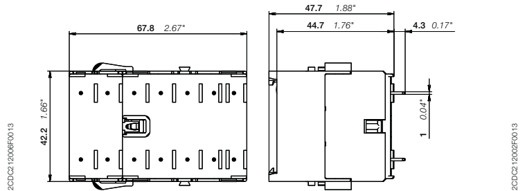
Mini contactors or contactor relays + CA6-11E-P, CA6-11M-P, CA6-11N-P
