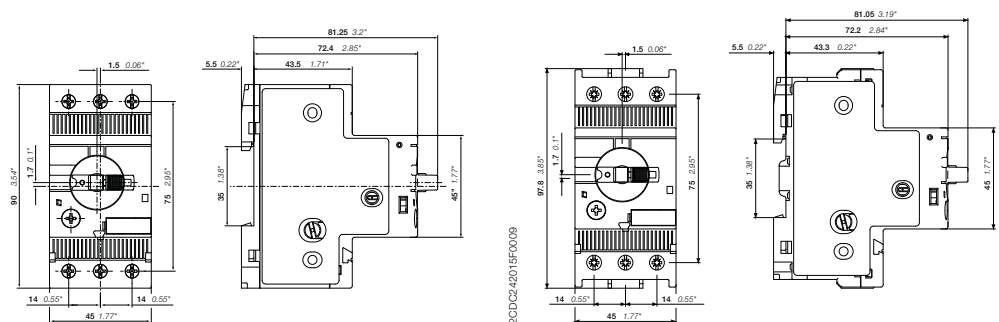
MS132T ≤ 10 A
