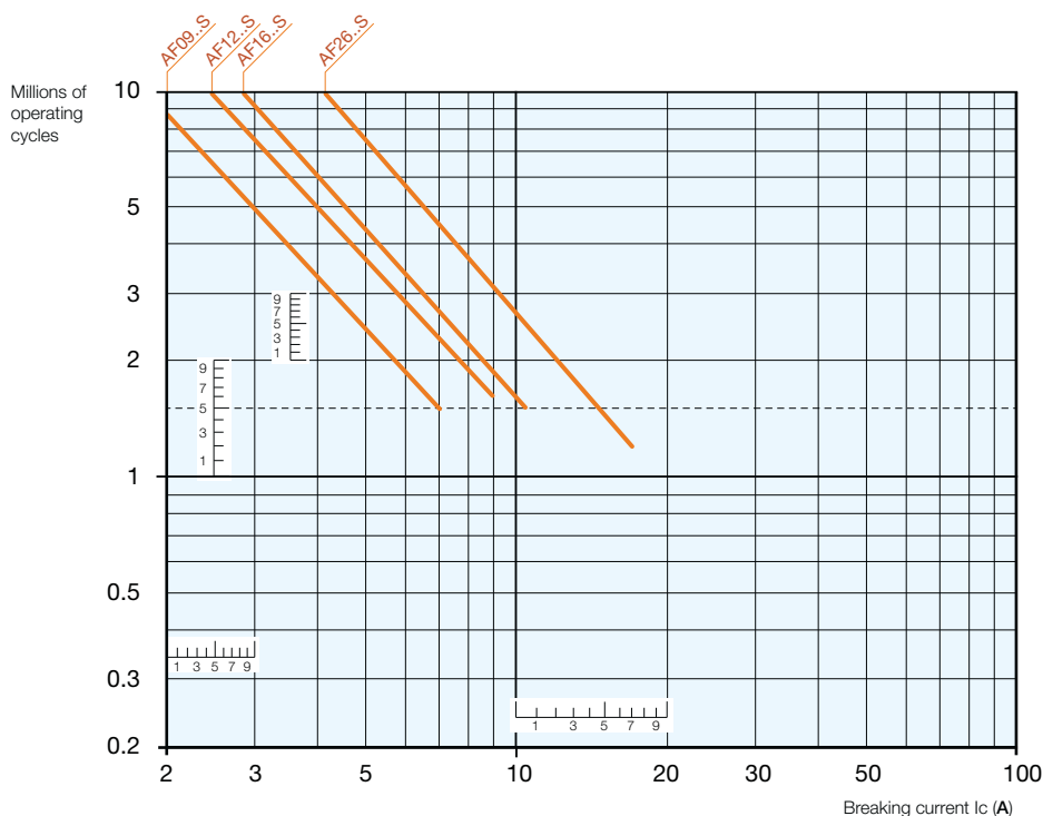
AF09..S ... AF26..S 3-pole contactors AC-3 electrical durability for 440 V < U_e \leq 690 V
