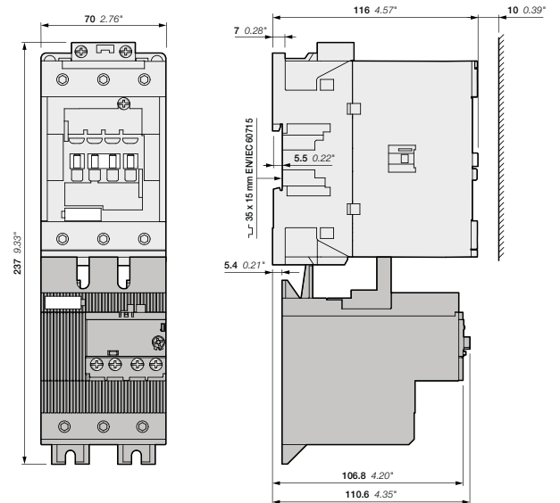
AF80, AF96 + EF96 electronic overload relay
