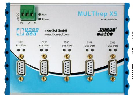
MULTirep X5 – 105 mm
