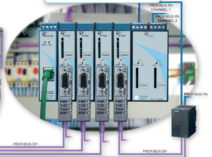
Modular data logger INBLOX®
