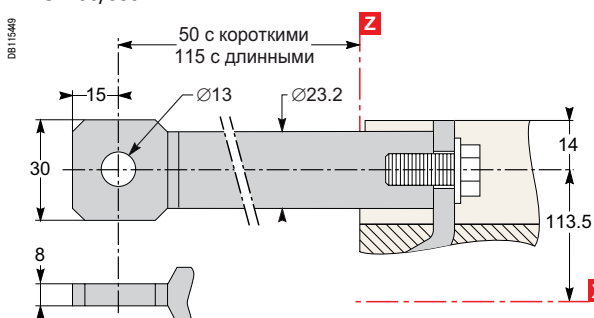
NSX400/630
