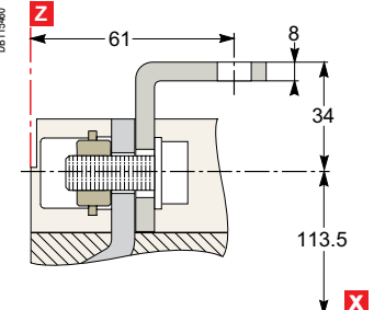
NSX400/630
