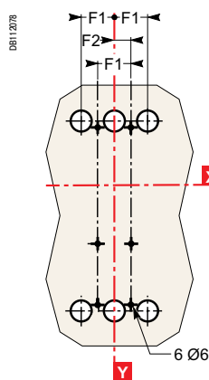
NSX400/630
